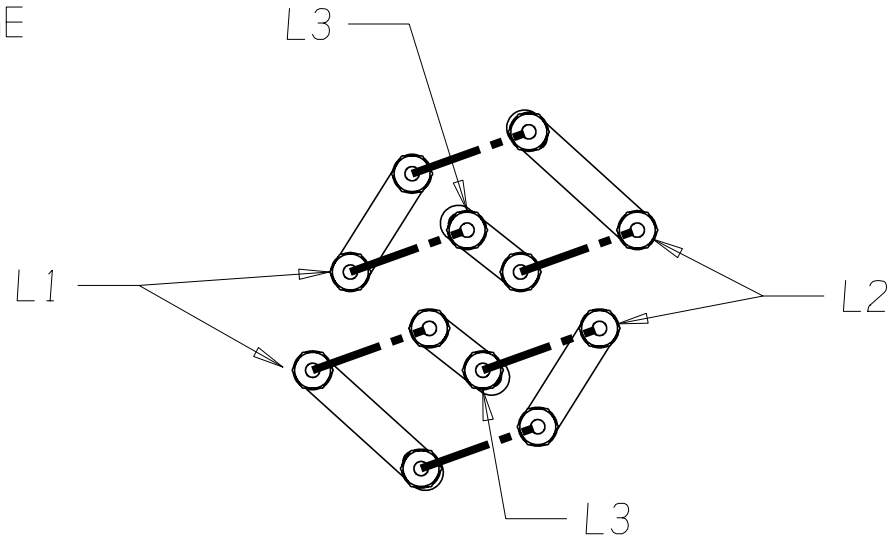
"K" CONFIGURATION WHEN USING 2 CONTACTORS
